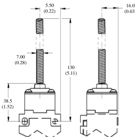
Top Wobble, Coil Spring
