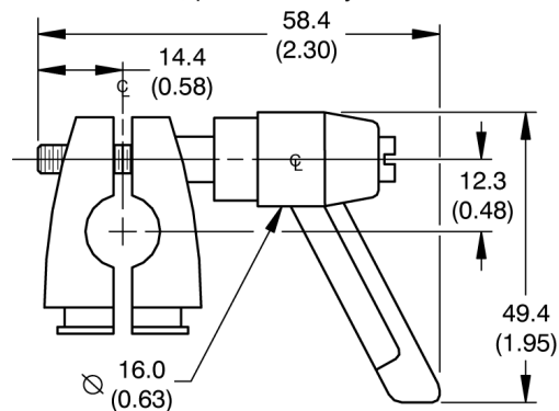
Model: SMS-HK-H Zinc cast, plated w/ Polyamide Handle
