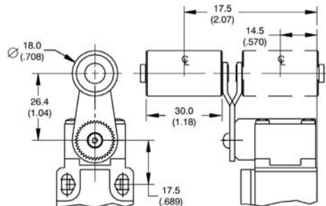
Side Rotary, Wide Roller Lever
