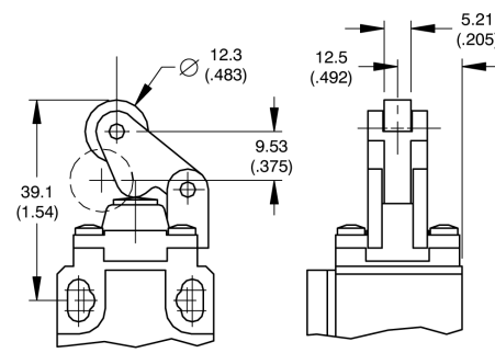
Top Push, Roller Lever
