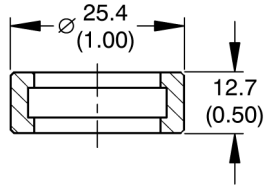
Coupler
