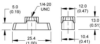
Rail Nut Model No. BMS-RN-1/4-20
