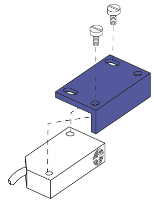
Angled style Housing Shields
