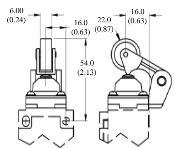
Top Push, Roller Lever
