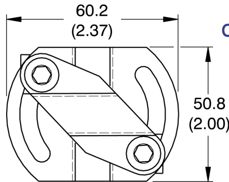
Model: SMS-CCR Stainless steel
